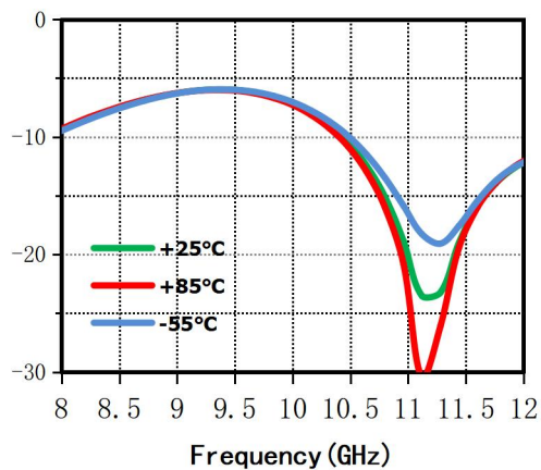
RF Input Return Loss (dB) vs.Temperature
