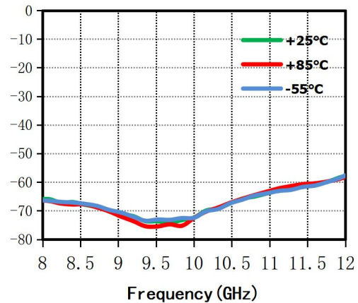
Isolation(dB) vs.Temperature
