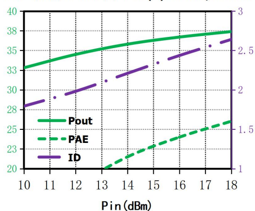
Pout (dBm), PAE (%), ID(A) vs. Pin, f=8GHz
