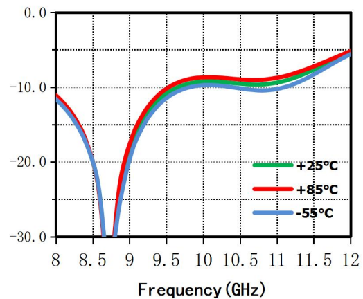
RF Output Return Loss(dB) vs.Temperature
